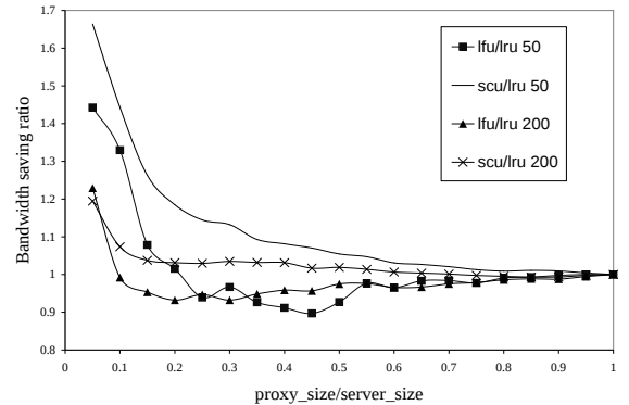
Figure 5: Impact of Object Number
